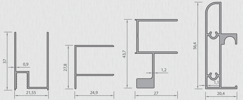
6090 GLASS PROFILE 0,265 kg/mt
