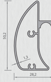
3864 RAIL PROFILE 0,536 kg/mt
