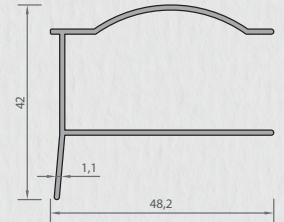
3097 DOOR STRIKE PROFILE 0,390 kg/mt
