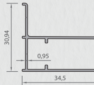
2373 WALL PILLAR PROFILE 0,274 kg/mt
