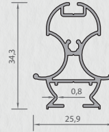
8508 CENTRAL PILLAR PROFILE 0,374 kg/mt
