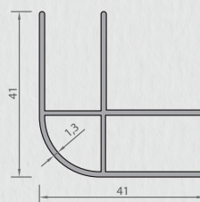
2384 ANGLED CONNECTED START PROFILE 0,521 kg/mt
