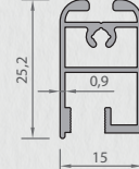
6472 PILLOW PROFILE 0,309 kg/mt
