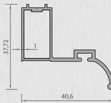
2366 SHORT DOOR STRIKE PROFILE 0,341 kg/mt
