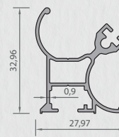
8509 CORNER BEAM PILLAR PROFILE 0,374 kg/mt
