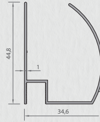
7389 GLASS PROFILE 0,355 kg/mt
